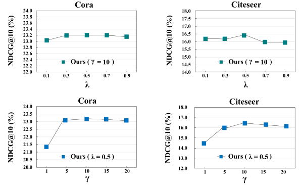
Figure 4: Hyper-parameters analysis on Cora and Citeseer.
