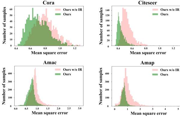
Figure 2: Effect of the information recomposing (IR) and affinity structure updating (ASU) schemes for node classification.
